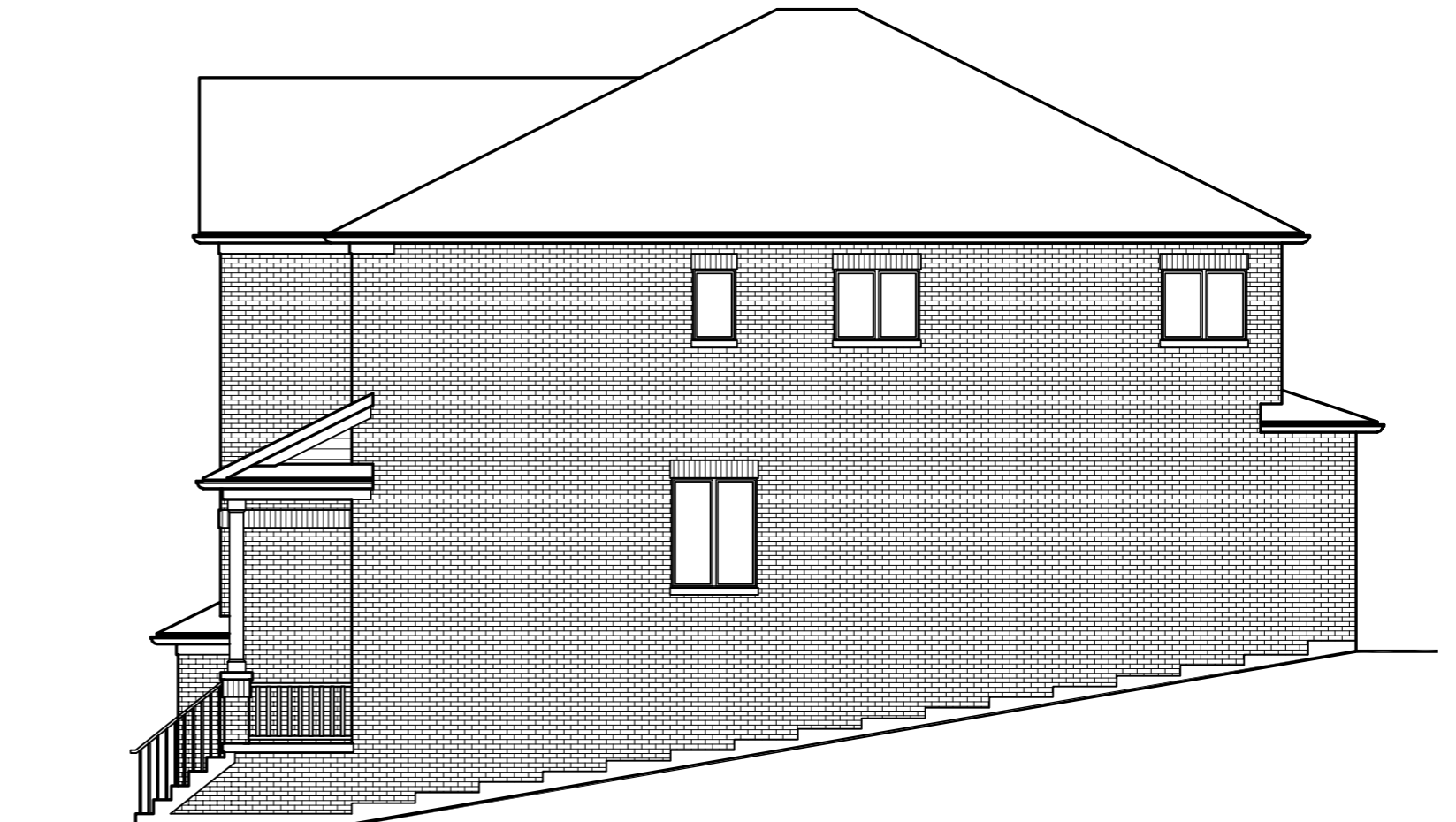
RIGHT SIDE ELEVATION 'A'
