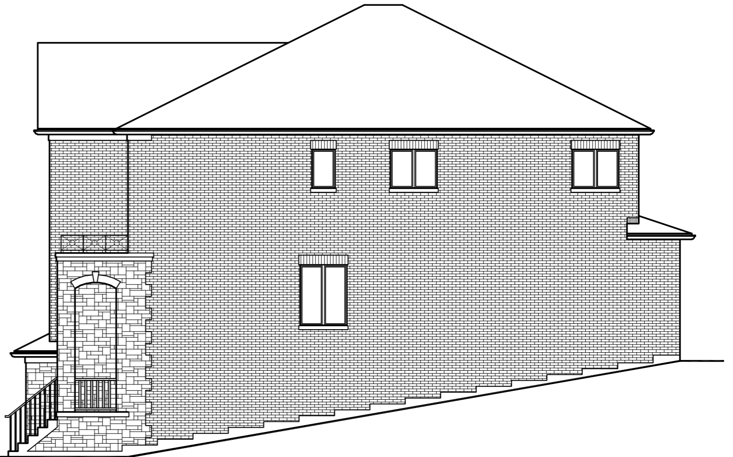
RIGHT SIDE ELEVATION 'B'
